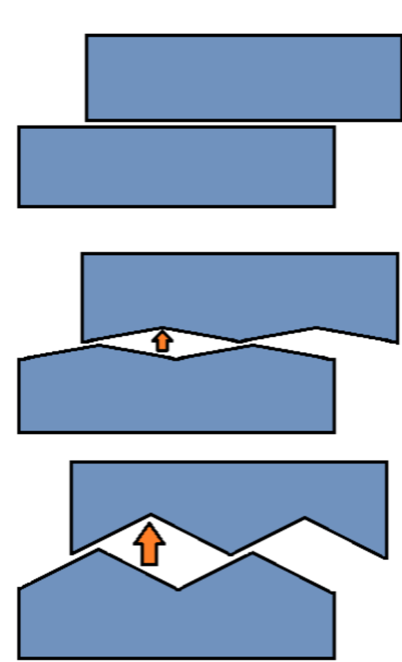
The amount of interpenetration between layers affects a plane's likeliness to slip (left). Identifying potential slip planes in a crystal structure (above)
